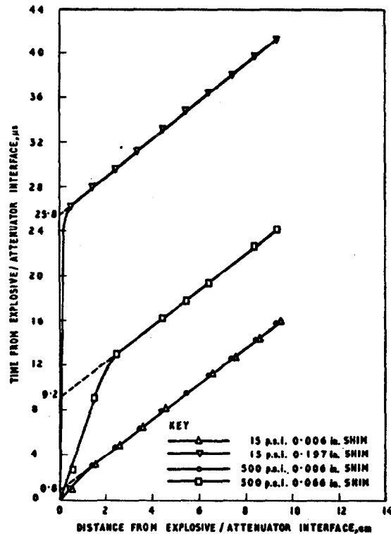
Fig. 12 Build-up to detonation in coarse HMX compacts at 1.14 g/cc filled with CH 4
